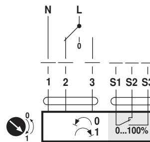
AC 230 V, 3-point
